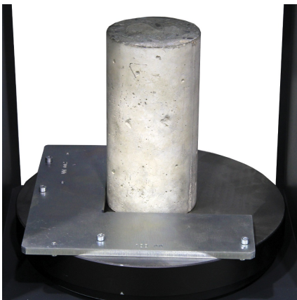
Model: 50-C0050/CTR2, centering device for 100mm, 150mm, 160mm and 200mm specimens suitable for frames and compression machines fitted with round plates 300mm dia.
