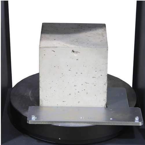
Model: 50-C0050/CTR2, centering device for 100mm and 150mm cubes. Suitable for compression plate 300mm dia.
